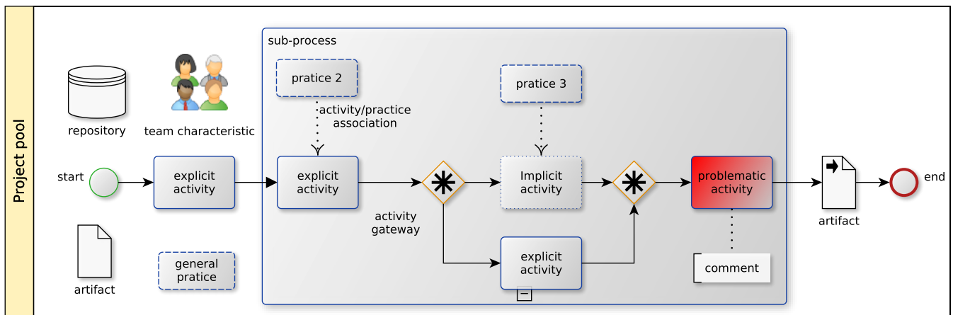
Figure 2: BPMN meta-model.
