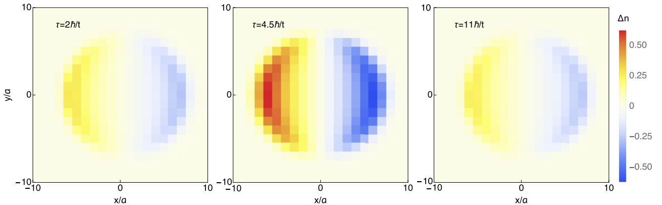
FIG. 5. The disorder-averaged local-density deviation from the initial state, \Delta n_i \equiv \langle \langle n_i \rangle \rangle_\tau - \langle \langle n_i \rangle \rangle_{\tau=0} , plotted as a function of position in the x – y plane for three different times. All model parameters are the same as in Fig. 4(a), where a superfluid occupies nearly the entire trap. These parameters correspond to the right arrow in the phase diagram in Fig. 2. Here we see how the superfluid as a whole oscillates in the trap even in the presence of disorder.
