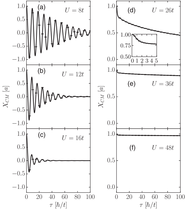
FIG. 4. The disorder-averaged center-of-mass position along the x direction plotted as a function of time for various interaction strengths U . The trap shift is chosen to be \Delta R_0 = a , and other model parameters are the same as in Fig. 3. (a)–(c) are initially in the disordered superfluid state. In (d) the center of the system is initially in the Bose-glass state, whereas (f) is initially in the Mott state. The inset in (d) shows the short-time behavior. (e) is initially in an intermediate state. In (d)–(f), the center of mass has a nearly constant velocity for \tau \gg \hbar/t .
