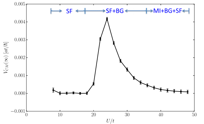
FIG. 9. The disorder-averaged center-of-mass velocity at long times [Eq. (10)] plotted as a function of interaction strength. For weak interactions the entire system is in the superfluid (SF) phase, and frequent center-of-mass oscillations result in a zero net velocity. For intermediate interaction strengths the Bose glass (BG) lies in the trap center. Here the two-step edge flow mechanism depicted in the right panel of Fig. 1 allows a small but finite center-of-mass velocity. At large interaction strengths the center of the system is in the Mott regime (MI), where tunneling into the edge (and therefore the center-of-mass velocity) is strongly suppressed.
