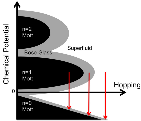
FIG. 2. Schematic mean-field phase diagram of the disordered Bose-Hubbard model [Eq. (1)] in the absence of a trap, \Omega = 0 . The black regions indicate the incompressible Mott insulators found at integer densities. The gray regions indicate the compressible Bose glass that separates the Mott from the superfluid. The three vertical arrows depict how the trapping potential lowers the local chemical potential as we move from the center of the system (top of the arrow) to the edge (bottom of the arrow). The three arrows represent regimes studied here, where the center of the system contains a disordered Mott insulator (left), Bose glass (center), and disordered superfluid (right).
