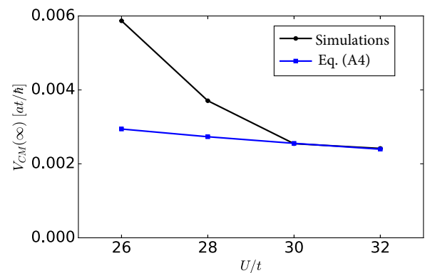
FIG. 11. Comparison of the center-of-mass velocity at long times between the estimate of the two-site model and numerical simulations for various interaction strengths.
