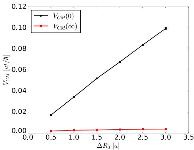
FIG. 7. The disordered-averaged center-of-mass velocity at short times [Eq. (9)] and long times [Eq. (10)] plotted as a function of the trap shift for an interaction strength of U = 26t . For short times, the center-of-mass velocity responds linearly to the length of the trap shift. For long times, the center-of-mass velocity barely changes with the trap shift.
