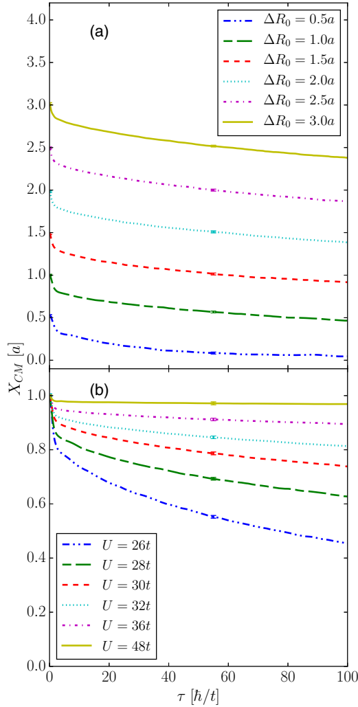
FIG. 8. The disorder-averaged center-of-mass position plotted as a function of time for (a) several different trap shifts U = 26 and (b) several different U for \Delta R_0 = a . The model parameters are otherwise the same as in Fig. 3. In (a) we see that different trap shifts do not change the long-time center-of-mass velocity (the slope is nearly constant). But in (b) we see that the slope depends on U .
