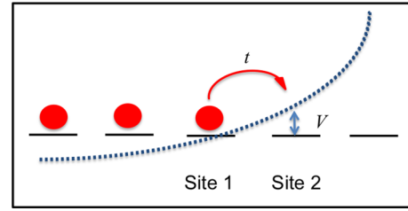
FIG. 10. Schematic showing sites of a lattice (dashes) along one direction filled up to site 1 with particles. Site 2 is an empty edge site. Tunneling from site 1 to site 2 is controlled with a potential V at site 2. The dotted line depicts the parabolic trapping potential which zeros the edge density.
