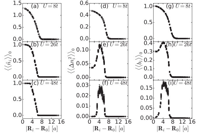
FIG. 3. (a)–(c) plot the disorder-averaged local density in the initial state as a function of distance from the center of the trap. (a) and (c) have a superfluid and Mott insulator in the trap center, respectively. (b) is in an intermediate regime. Model parameters are chosen to be disorder strength \Delta = 0.3U , trap strength \Omega = 0.02U , and central chemical potential \mu = 0.5U . (d)–(f) plot the same but for the disorder-averaged local-density fluctuations in the initial state. The density fluctuations in (e) and (f) show the edge superfluid. (g)–(i) plot the disorder-averaged local superfluid order parameter in the initial state. Error bars result from disorder averaging.
