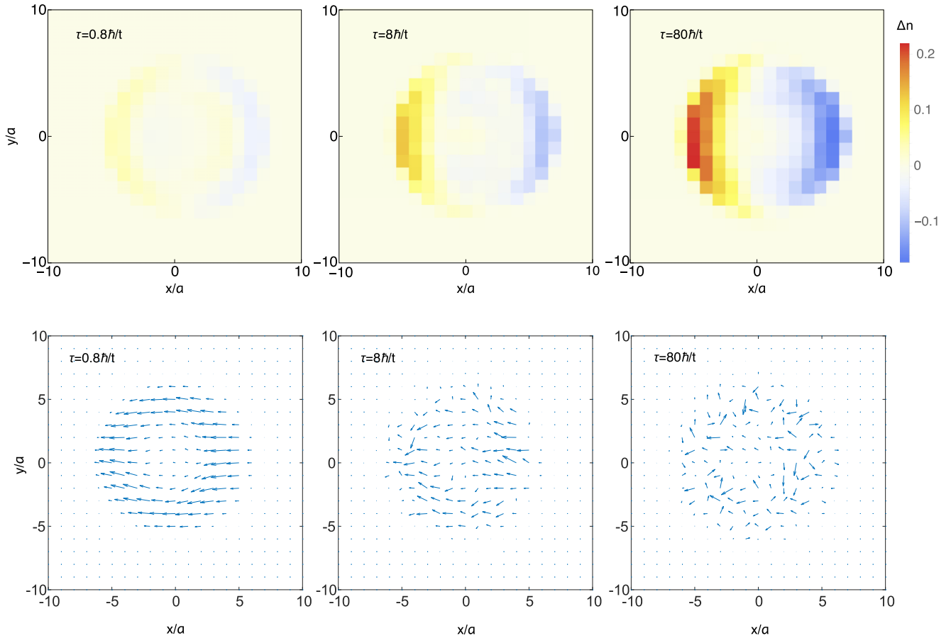
FIG. 6. Top: the same as Fig. 5 but for an interaction strength of U = 26t [parameters in Fig. 4(d)], which corresponds to a Bose glass in the center of the trap (central arrow in Fig. 2). Bottom: the disorder-averaged local current flow with the same parameters as in the top panel. At \tau = 0.8\hbar/t we see the first mechanism of transport where at short times the edge state quickly slips around the central insulator, depicted in the left panel of Fig. 1. At \tau = 8\hbar/t and 80\hbar/t we see a different two-step mechanism of transport, depicted in the right panel of Fig. 1. Here the particles first slowly tunnel out of the central insulator to get pushed, in the second step, quickly along the edges. In the two right snapshots, lateral tunneling events and a shrinking of the central insulator can be seen.
