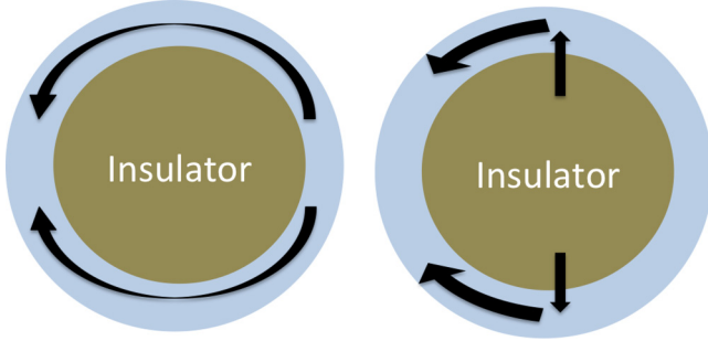
FIG. 1. Schematic showing two distinct mechanisms for center-of-mass dynamics after an initial shift of the trapping potential to the left. The center of the system is in an insulating phase (either the Mott insulator or the Bose glass), but the edges are superfluid. Left: We find that initially (on times scales shorter than the intersite tunneling), the edge superfluid quickly moves around the insulator to the left to redistribute the total center of mass. Right: We find that (on time scales much larger than the intersite tunneling) a two-stage process shifts the center of mass. First, particles slowly tunnel out of the central insulator into the edges (vertical arrows). Then the particles quickly move to the left along the edge to redistribute the center of mass.
