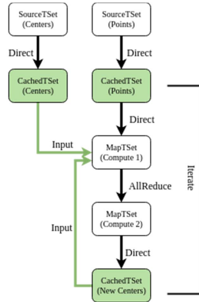
Fig. 3. K-Means TSet API dataflow graph.
