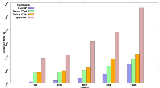
Fig. 4. K-Means job execution time on 16 nodes with varying centers, 2 million data points with 128-way parallelism for 100 iterations.
