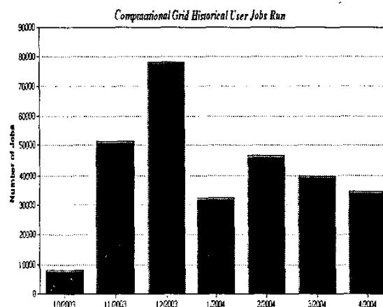
Figure 6 Distribution of the number of jobs run on Grid3 by month starting from October 2003.
