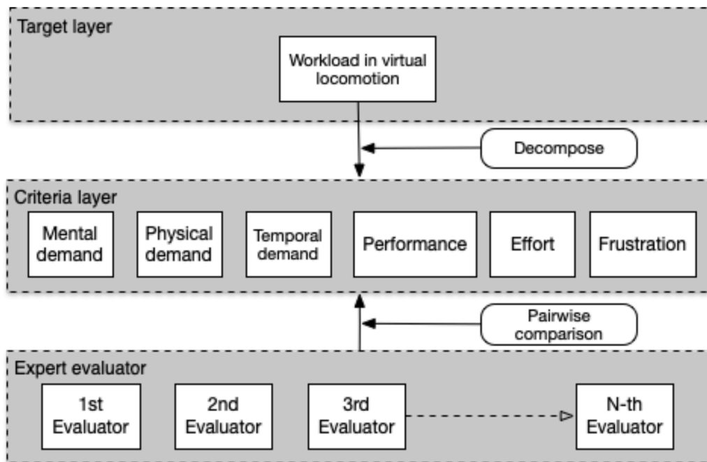
Fig. 2. A specific case of hierarchical structure to measure workload with the NASA-TLX criteria.
