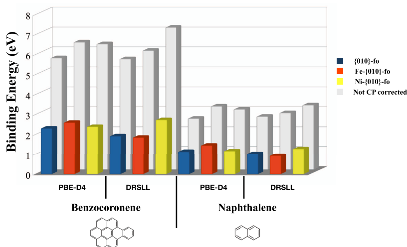
Figure 8. Binding energies of benzocoronene and naphthalene chemisorbed on {010}-fo (singlet), Fe (quintet), and Ni-{010}-fo (triplet) surfaces using PBE-D4 and DRSL with the CP-DZP basis set and with the corresponding counterpoise-noncorrected values at the back. The order of the labels of the forsterite surfaces corresponds to the order of the bars. Note: Numerical values are reported in the SI.
