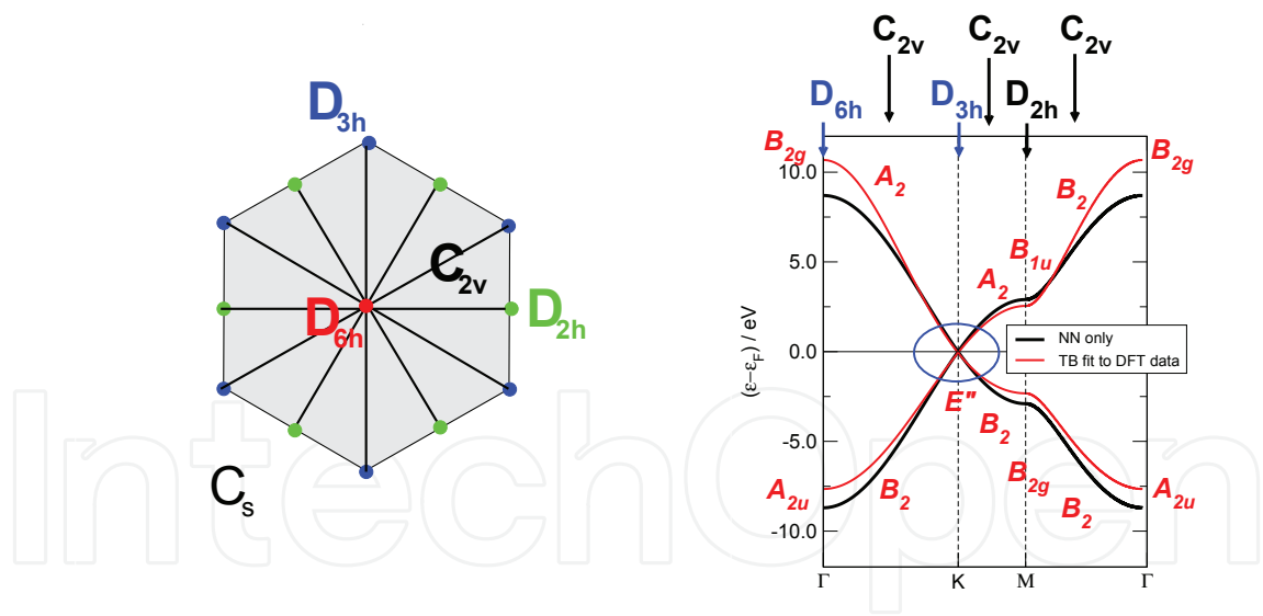
Fig. 3. Left panel: point-symmetry classification of Bloch states in graphene. k -groups are color coded as indicated. Right panel: symmetry labels for graphene electronic states on the highest-symmetry lines of the BZ.
