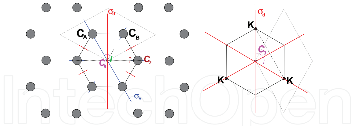
Fig. 2. Left panel: Point symmetry elements in graphene lattice. Reflection planes orthogonal to the page, \sigma_v and \sigma_d , are replicated by the six-fold rotation axis C_6 , along with the two-fold rotation axis on the page plane, C_2 . I is the inversion center, at the center of the Wigner-Seitz cell (solid line). The page plane is, of course, a reflection plane ( \sigma_h ). Right panel: symmetry elements of the k -group at the K point ( D_{3h} ). Black dots mark the K point and its images.
