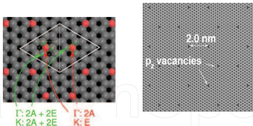
Fig. 12. Left: counting the number of irreps generated by the atomic basis in a 4x4 supercell: indicated are the irreps generated by the atoms at the center of the half-cells (red balls) and by green triangles. Right: a simple “supergraphene”, the simplest defective 14x14 honeycomb.
