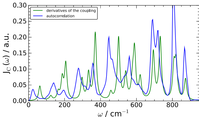
FIG. 4. The spectral density of the coupling on the carbon atom J_C(\omega) as computed from the analysis of the source potential (green line, see text for detail). Also shown for comparison, the trajectory-based spectral density reported in panel (c) of Fig. 3 (blue line, T = 5 \text{ K} ).
