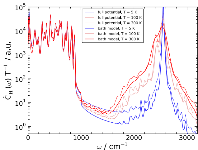
FIG. 7. Temperature scaled position autocorrelation function of the hydrogen atom C_H(\omega)T^{-1} as computed with the lattice model (thin lines) and the derived IO model (thick line), at three different temperatures T = 5 K, 100 K, and 300 K. The IO model used the T = 5 K spectral density J_C(\omega) shown in Fig. 3, truncated at \omega_D = 1000 \text{cm}^{-1} .
