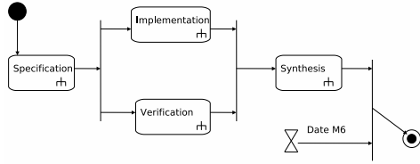
Figure 1: The workflow definition following SciWay 2.0.
