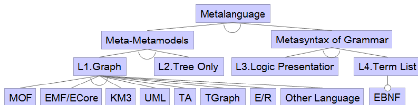
Fig. 10 Feature diagram for the metalanguages
