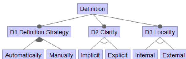
Fig. 13 Feature diagram for the definition
