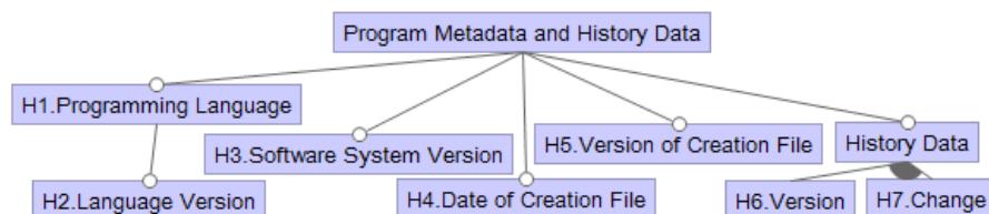
Fig. 14 Feature diagram for the program metadata and history data
