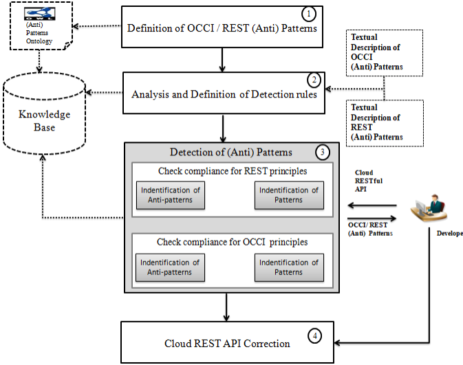
Fig. 2: Approach overview
