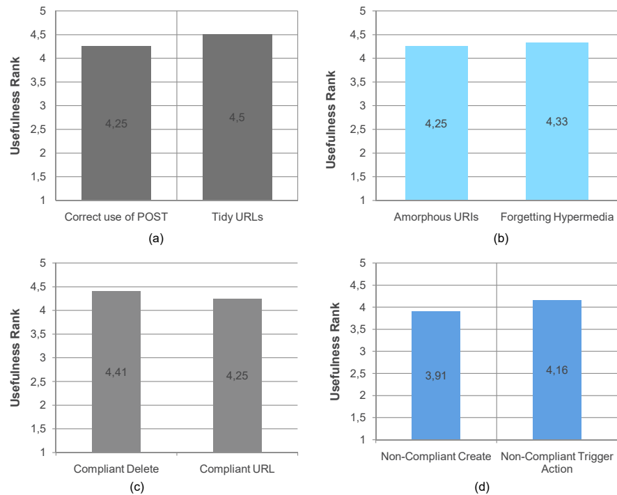
Fig. 8: Usefulness Detection Rate for (a) REST patterns: Correct use of POST, Tidy URLs ; (b) REST anti-patterns : Amorphous URIs, Forgetting Hypermedia ; OCCI patterns: Compliant Delete, Compliant URL ; OCCI anti-patterns: Non-Compliant Create, Non-Compliant Trigger Action
