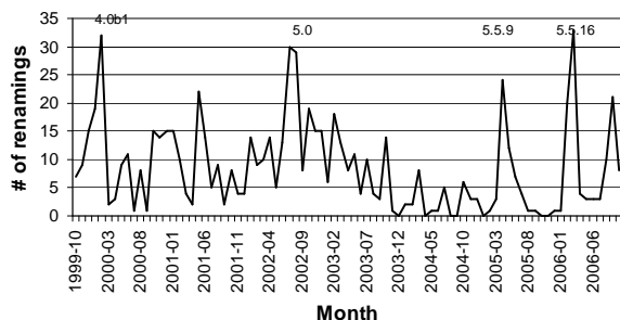
(b) Tomcat
