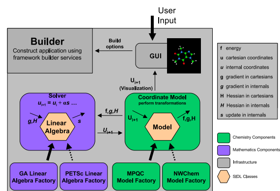
Figure 2. The high-level component architecture for NWChem and MPQC courtesy of Curtis Janssen and Joseph P. Kenny, Sandia National Laboratories
