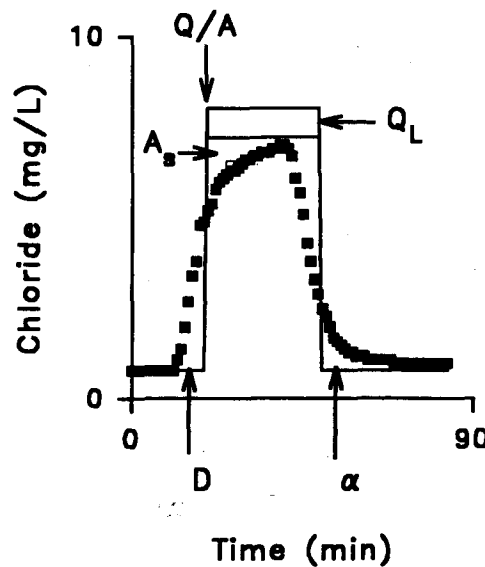
FIG. 2. Example chloride curve produced from samples collected at a downstream site. The height, width, and arrival time of the square wave are determined by the concentration and duration of the solute release, and velocity of the water. Additional parameters smooth the square wave into a curve. Parameters are positioned according to the region of the curve they most strongly influence. Q = discharge, A = stream cross-sectional area, Q/A = velocity, Q_L = lateral inflow, D = dispersion, A_s = transient storage zone cross-sectional area, and \alpha = transient storage coefficient.
