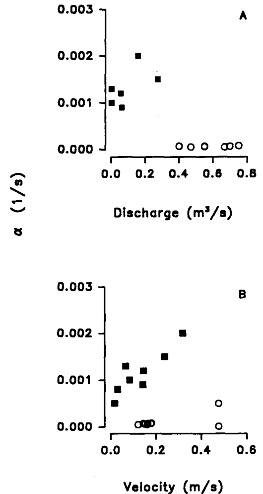
FIG. 7. A.—Correlation between exchange coefficient ( \alpha ) and discharge for all 1st- through 5th-order sites. Overall r was -0.42 ( p < 0.05 , n = 13 ). Alpha and Q were not correlated for 1st- through 4th-order Coweeta sites (filled squares) or 5th-order H. J. Andrews sites (open circles) when evaluated separately. B.—Correlation between the exchange coefficient ( \alpha ) and velocity was not significant for 1st- through 5th-order sites overall, or for 5th-order sites (open circles) evaluated separately. The correlation was significant ( r = 0.82 , p < 0.04 , n = 8 ) for 1st- through 4th-order Coweeta sites (filled squares).
