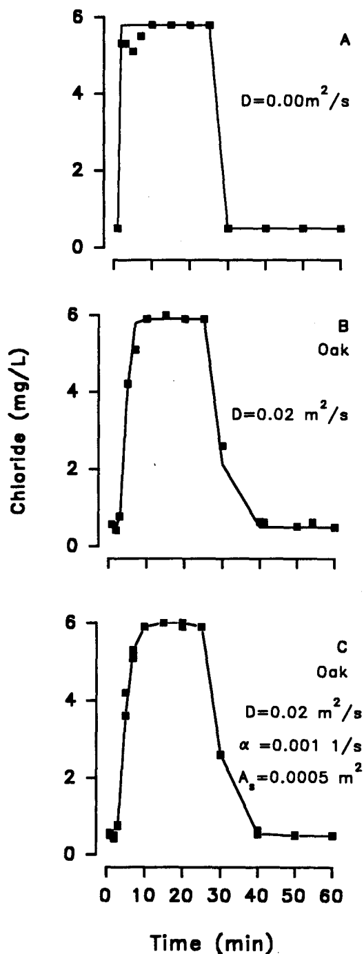
FIG. 3. A.—Model simulation (line) without transient storage compared with chloride data (squares) for an artificial stream in November 1987 when no leaves were in the streams. B.—Model fit when leaves had been in the streams for about four months (March 1988). C.—Model fit to the same data as B with transient storage included. Symbols as in Figure 2.
