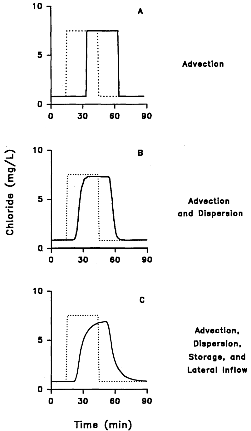
FIG. 1. Theoretical representation of a chloride curve from an upstream site, and model simulation of a downstream site depicting the shape of the solute curve with advection only (A), advection and dispersion (B), and advection, dispersion, transient storage and lateral inflow (C). Dotted lines represent the upstream curve (at the top of the release site) and solid lines represent the downstream curve (at the bottom of the release site).
