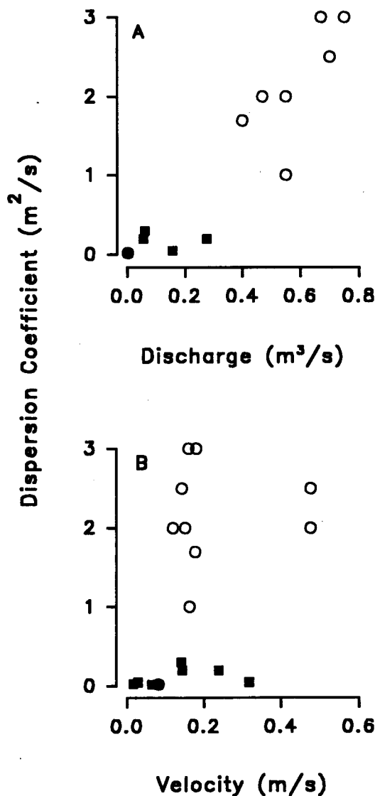
FIG. 4. A.—Correlation between dispersion and discharge for 1st- through 4th-order stream sites (filled squares) and 5th-order stream sites (open circles) ( r = 0.92 , p < 0.0002 , n = 12 ). B.—Correlation between dispersion and velocity for 1st- through 4th-order stream sites (filled squares) and 5th-order stream sites (open circles) ( r = 0.51 , p < 0.03 , n = 17 ).
