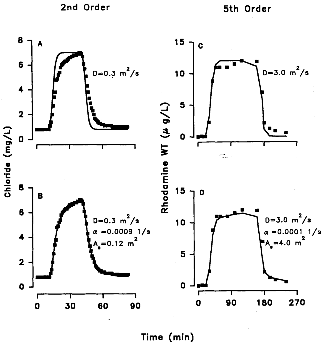
FIG. 5. A.—Model simulation (line) without transient storage compared with chloride data (squares) for a 2nd-order site on Ball Creek at the Coweeta Hydrologic Laboratory, July 1991. B.—Model fit to the data in (A) when transient storage is included. C.—Model simulation without transient storage compared with rhodamine WT data for a 5th-order stream at the H. J. Andrews Forest, September 1987. D.—Model fit to the data in (C) when transient storage is included. Symbols as in Figure 2.
