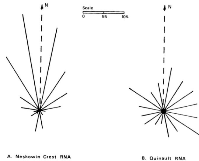
Fig. 13. Orientation of logs in two Picea sitchensis - Tsuga heterophylla forests from the northwestern United States. The length of the lines indicates the percentage of logs pointing in a given direction. (A) Neskowin Crest Research Natural Area, Oregon. (B) Quinault Research Natural Area, Washington. In spite of similar canopy composition, the logs at Neskowin Crest have a strong northerly orientation, while those at Quinault have a fairly random orientation pattern.
