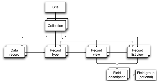
Figure 7: Annalist internal data model.
