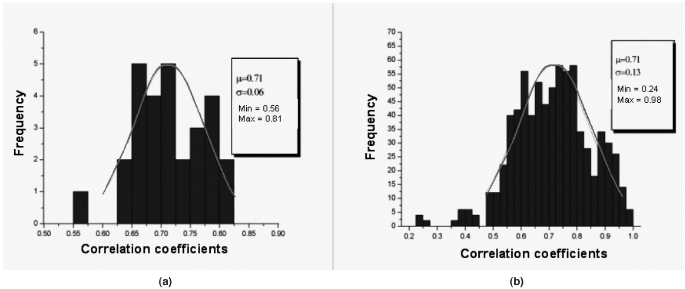
Figure 7. a) Histogram of the correlation coefficients between features and the 'defect' and 'regular structure' classes b) histogram of correlation coefficients between features
