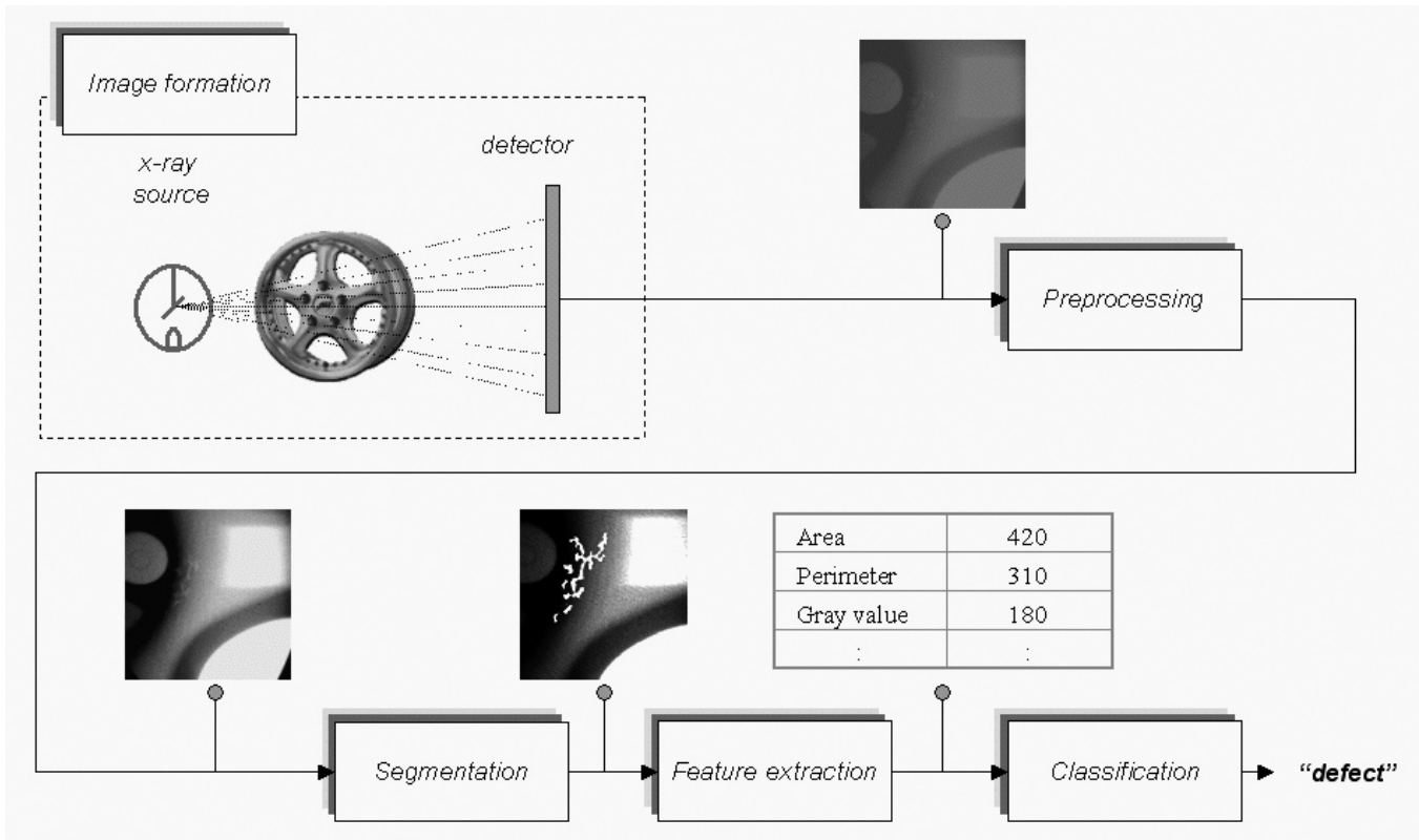
Figure 1. Pattern recognition in the automatic detection of flaws
