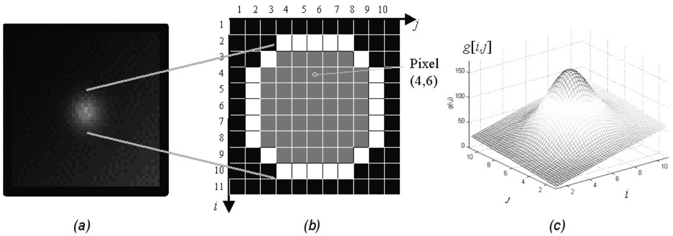
Figure 3. Example of a region. (a) X-ray image, (b) segmented region, (c) 3d representation of the intensity (grey value) of the region and its surroundings
