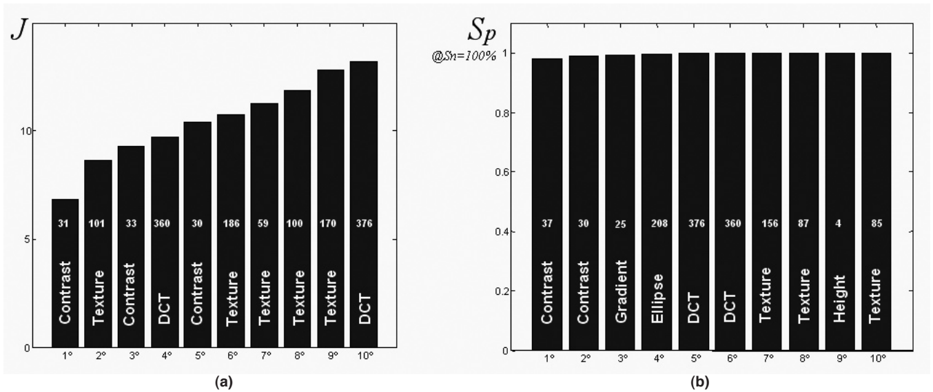
Figure 6. Selection of the first 10 features 10 by means of the SFS method using a) Fisher discriminator ( J ) and b) sensitivity specificity = 100%
