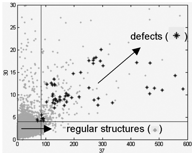
Figure 8. Vector space of features F_1 (# 37) and K_c (# 30), the lines represent the thresholds
