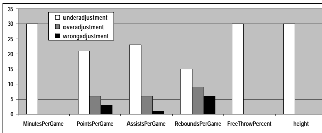
Figure 3: Comparing under adjustments, over adjustments, and wrong adjustments made by Knack over all the estimation problems.
