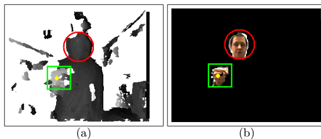
Fig. 3. Hand detection and segmentation: (a) Unsegmented depth image showing face detection (red circle) and nearest point detection (yellow dot), with estimated hand scale (green box). (b) Hand and face appearance after background suppression via depth.
