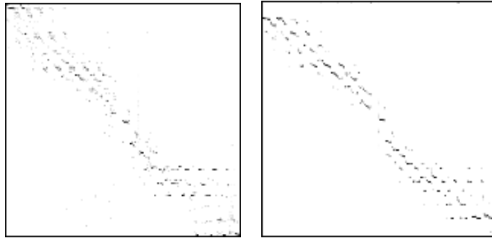
Fig. 7. Confusion matrices, (a) without and (b) with pose tracking, for the 153 class head pose task. Darker pixels indicate greater classification rates. The average correct classification rates (within 10 degrees) are 47%, and 64% respectively
