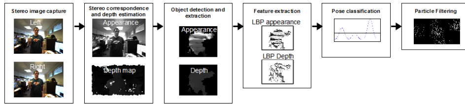
Fig. 1. Proposed framework, for real time, generalised pose estimation. Example appearance and depth images are included at each stage.
