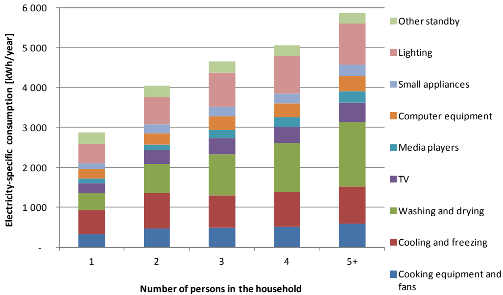
Figure 3.9 Electricity consumption in households of different sizes (Xrgia, 2011)
