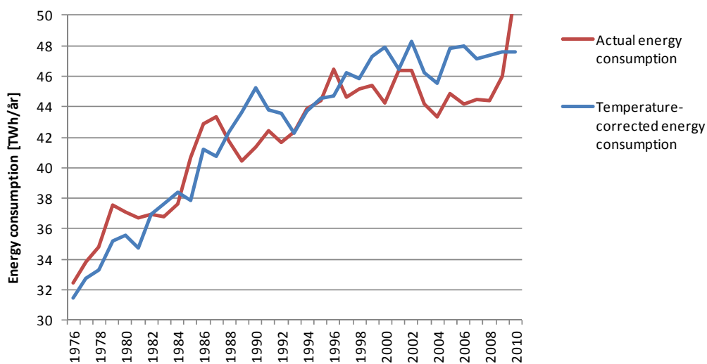
Figure 3.3 Trend in overall household energy consumption. (MET, 2012) (SSB, 2012)
