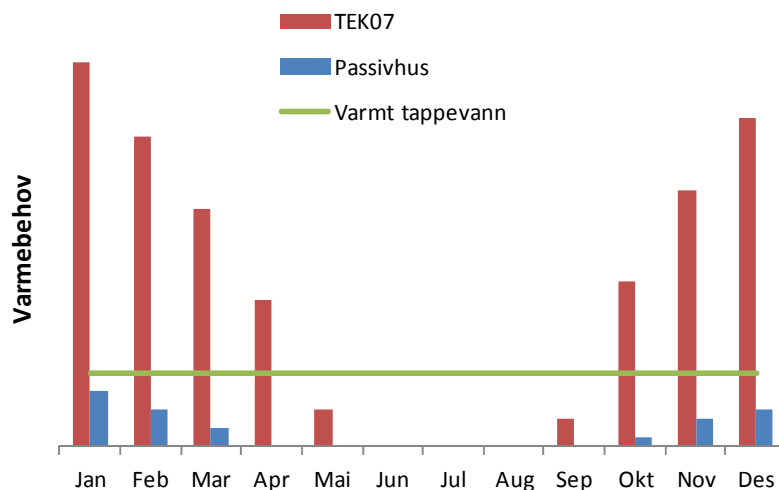
Figure 3.14 Energy requirements for space heating for TEK07 and passive houses, and hot water for a house in the Oslo climate (I.Andresen, et al., 2010).
