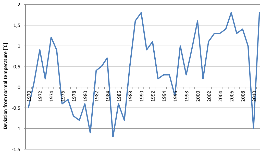
Figure 3.5 Deviations from normal temperatures, annual figures. Norway. (MET, 2012)
