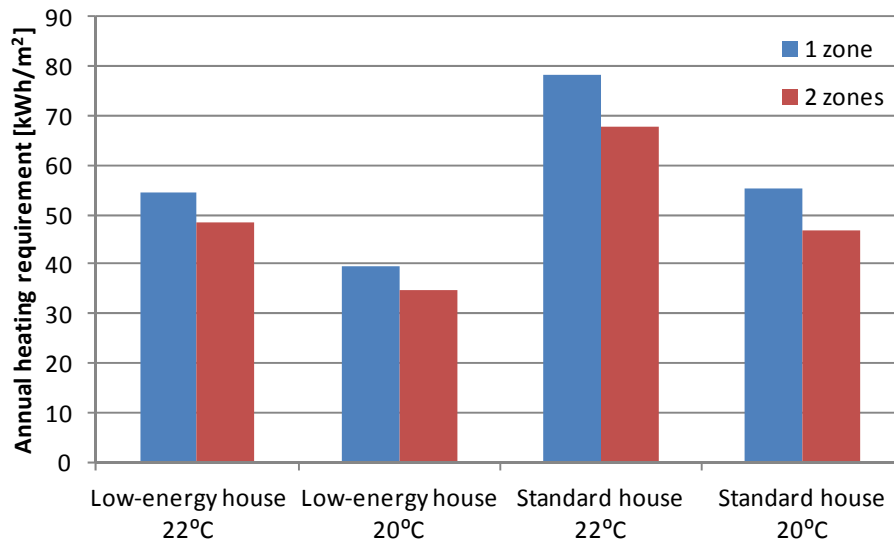
Figure 3.18 Reduced energy consumption from the introduction of temperature zones (Stieldorf, Juri, Haider, König, & Unzeitig, 2001)
