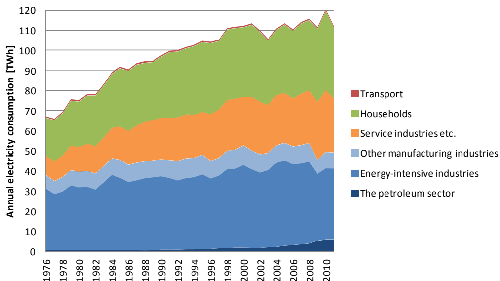
Figure 2.4 Electricity consumption in mainland Norway by sector. Source: NVE / (SSB, 2012)
