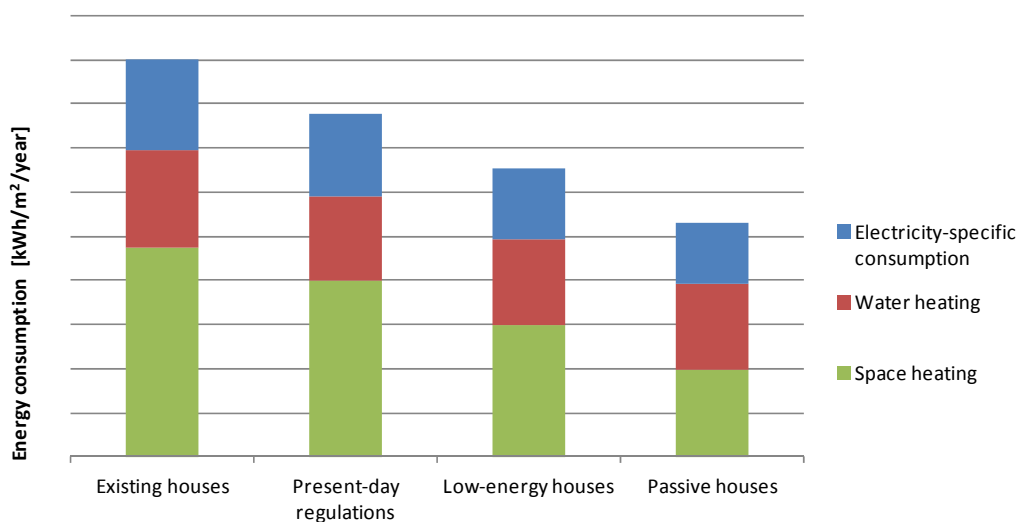
Figure 3.15 Typical energy consumption by end-use for houses built to different technical regulations
