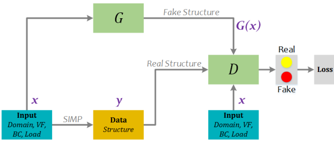
FIGURE 3. Baseline: cGAN for topology optimization.
