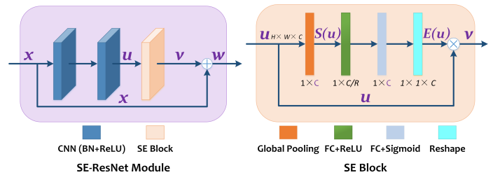
FIGURE 5. ResNet enhanced by SE block [58].
