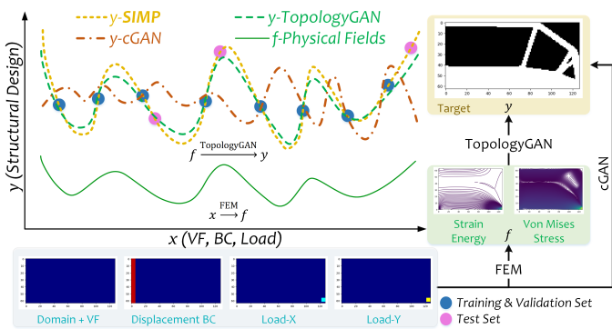
FIGURE 6. Schematic diagram of TopologyGAN.
