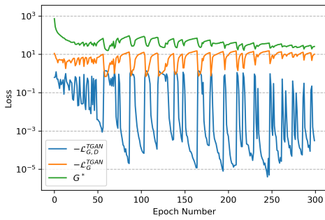
FIGURE 10. Loss functions of TGAN, Discriminator and Generator in training.
