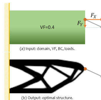
FIGURE 1. 2D topology optimization.
