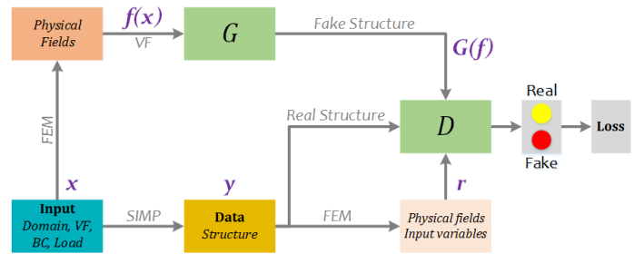
FIGURE 7. TopologyGAN approach to topology optimization.
