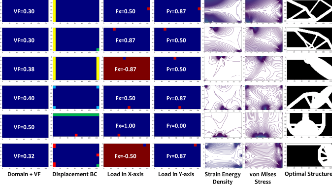
FIGURE 9. Data samples generated by FEM solver and SIMP solver. Images in each row form one sample. The first four images in each row are input variables x (VF,BC,Load), the last image is output y . Strain energy density and von Mises stress are shown in level sets with contour lines.
