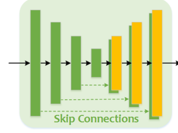
FIGURE 4. Architecture of the U-Net. The skip connections between networks are illustrated as dotted arrows.
