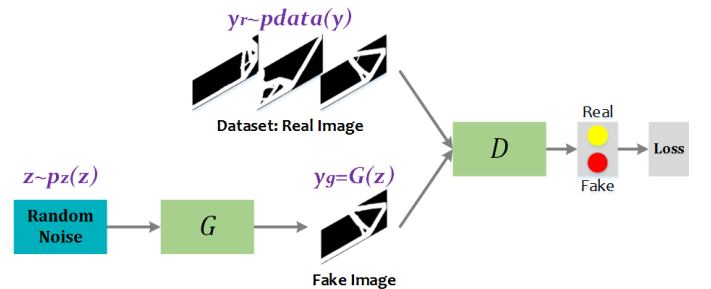
FIGURE 2. Schematic diagram of GAN.
