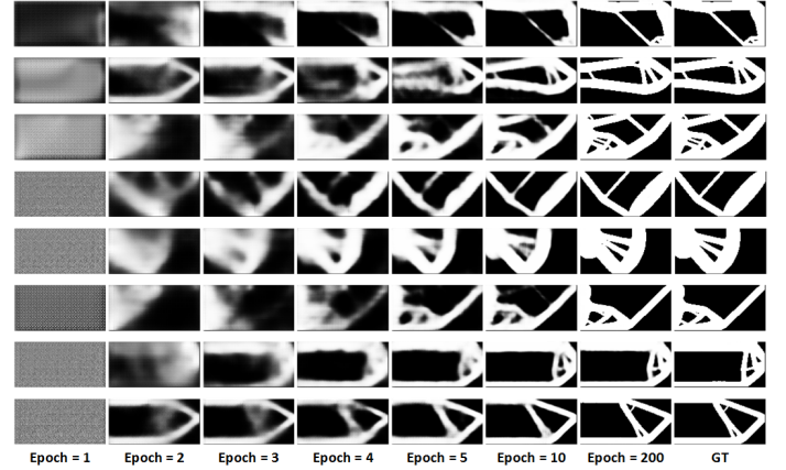
FIGURE 12. Evolution of TopologyGAN predictions during training.
