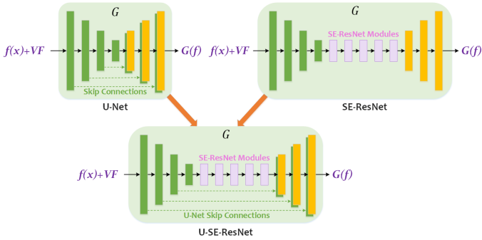
FIGURE 16. Architectures of U-Net, SE-ResNet, and U-SE-ResNet
