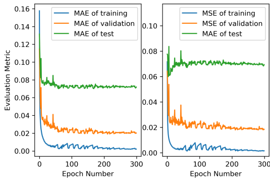
FIGURE 11. MAE and MSE of TopologyGAN in training.
