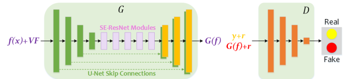
FIGURE 8. Architectures of the generator G and discriminator D .
