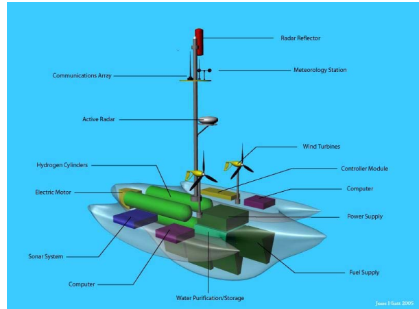
Figure 3. ASC Sea Rover concept vehicle. Courtesy NASA Ames Research Center, Jesse Haitt, UCSC.
