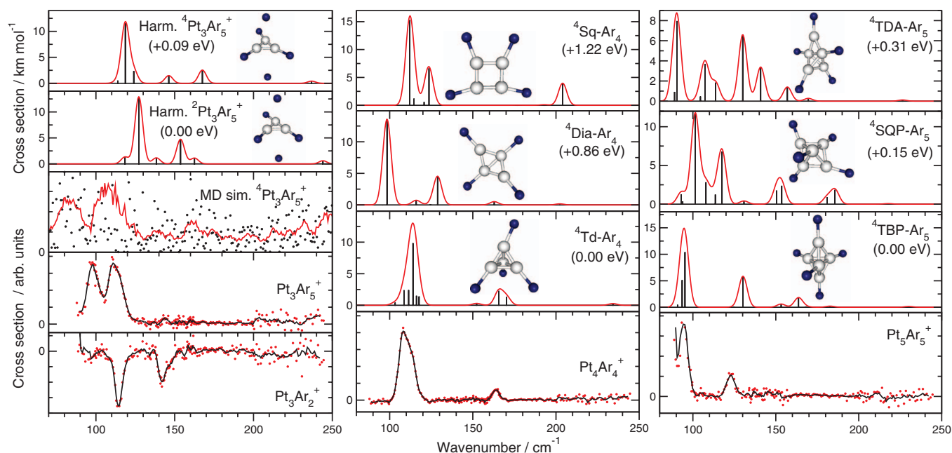
FIG. 1. Experimental and calculated spectra of Pt_n Ar_m^+ . (a) Pt_3 Ar_m^+ ; the experimental spectrum of Pt_3 Ar_5^+ shows growth due to fragmentation of clusters with more argon, below \sim 100 cm^{-1} the heating of the clusters appears to be insufficient to boil off three Ar atoms from Pt_3 Ar_5^+ , (b) Pt_4 Ar_4^+ and (c) Pt_5 Ar_5^+ . All of the harmonic spectra were calculated at the TPSS/def2-TZVP level, the relative energies are shown for the argon complexes. The leading superscripts show the spin multiplicity of the species.
