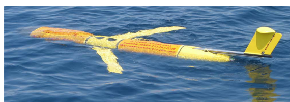
Fig. 9. Slocum Glider as used by the University of Southern California (courtesy of Smith et al. [47]).
